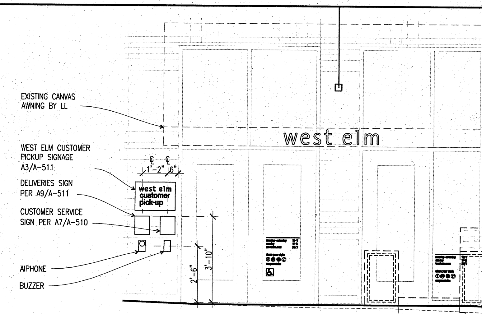
E7 CUSTOMER PICKUP - ENLARGED ELEVATION 3/8"=1'-0"
