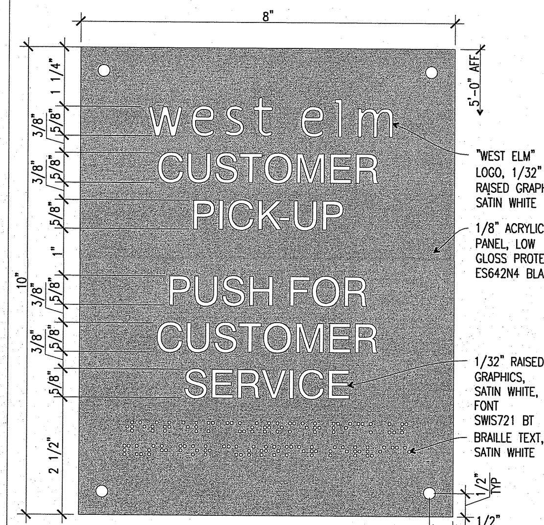
A7 CUSTOMER PICK-UP SIGNAGE 6"=1'-0" SIGNAGE F010
