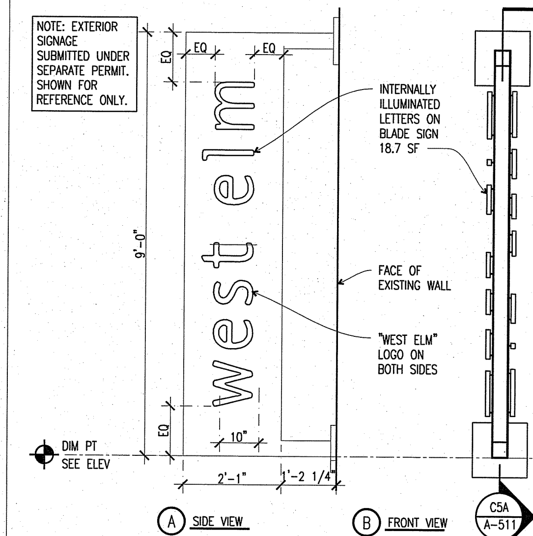
C9 ILLUMINATED BLADE SIGN 1/2"=1'-0"
