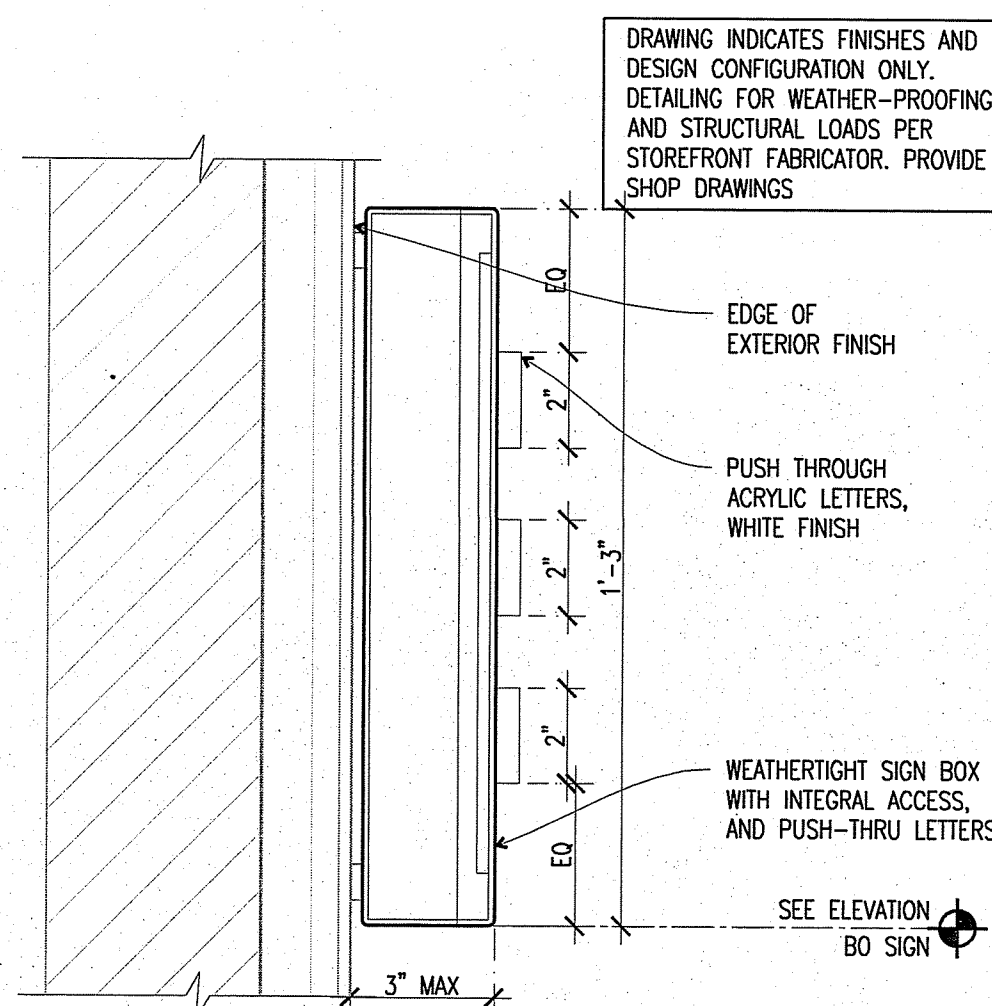
A1 SECTION AT CUSTOMER PICK-UP SIGN 3"=1'-0" SIGNAGE F010
